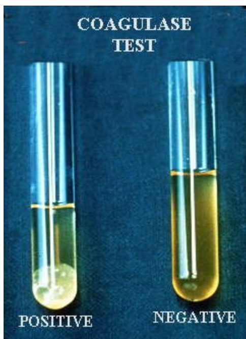
Coagulase Test
